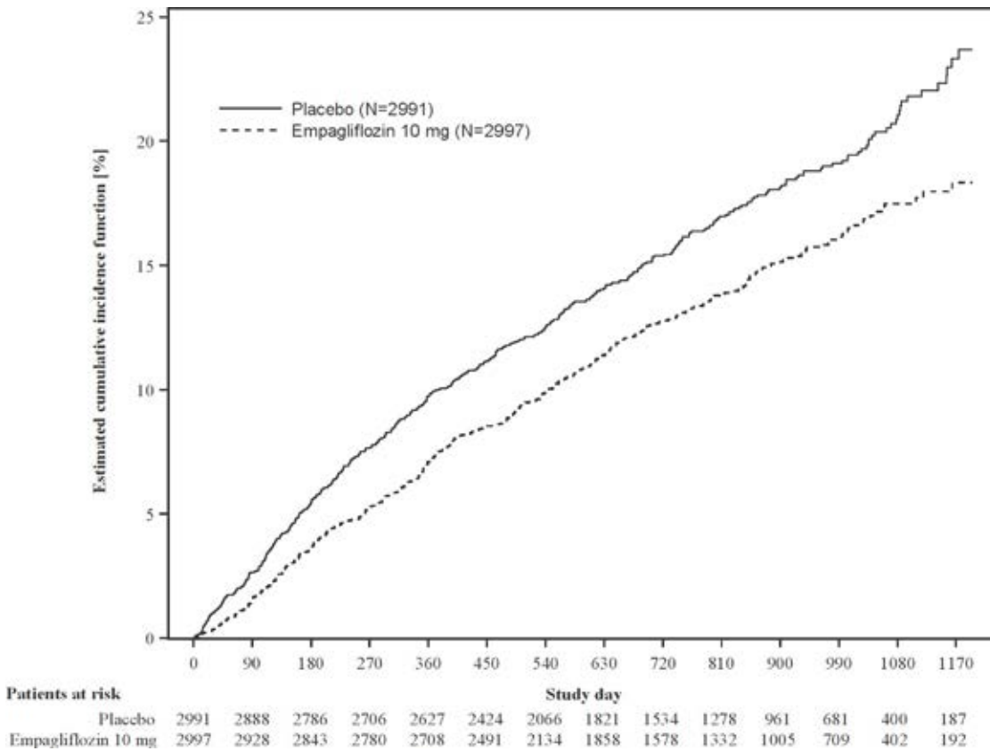
Figure 9 Time to first event of adjudicated CV death or HHF
