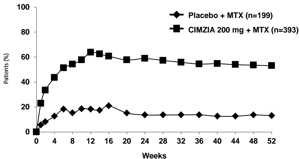
Figure 1 Study RA-I ACR20 Response Over 52 Weeks
