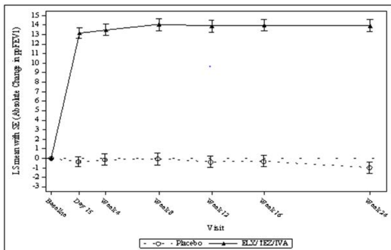
Figure 2: Absolute Change from Baseline in Percent Predicted FEV 1 at Each Visit in Study 445-102
