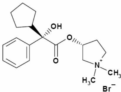
[2S, 3R]-stereoisomer
