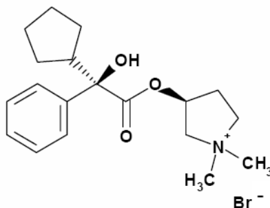
[2R, 3S]-stereoisomer
