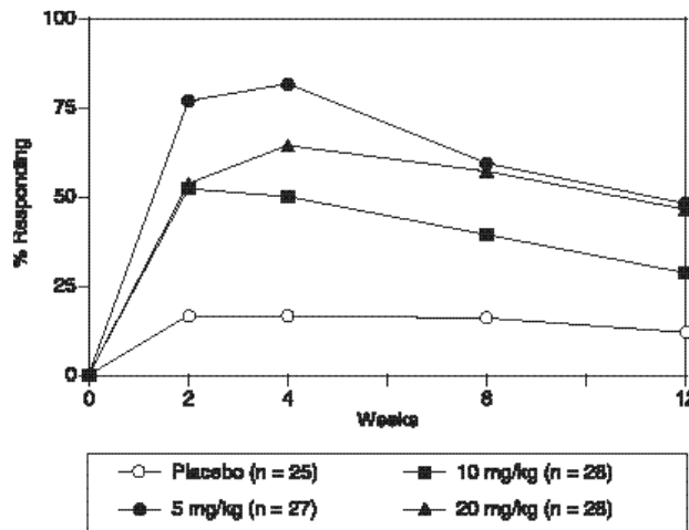
Figure 1. Response ( 3 70 point decrease in CDAI) to a Single IV infliximab or Placebo Dose
