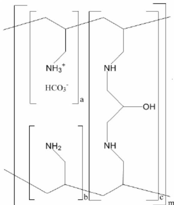
Figure 1 - Structure of sevelamer carbonate
